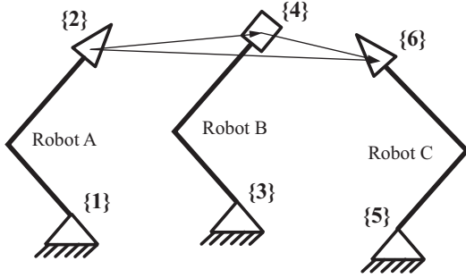
Fig. 2. An schematic diagram of a 3-arm parallel manipulator, with the corresponding reference frames and the relative position vectors.
