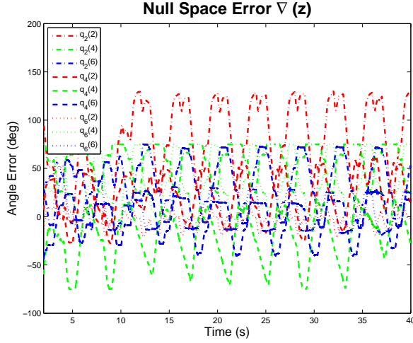
Fig. 10. The null space posture error \nabla(z) .
