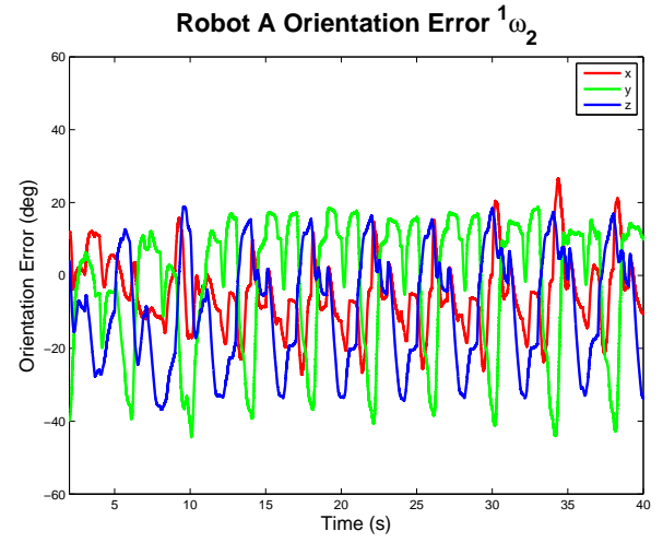
Fig. 7. The robot A orientation error {}^1\omega_2 .
