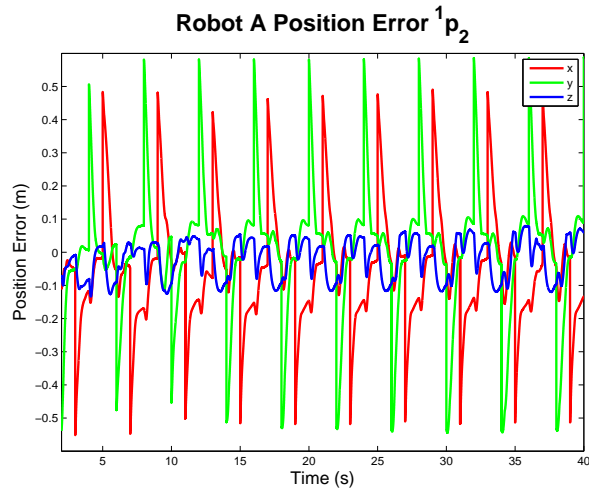
Fig. 6. The robot A position error {}^1p_2 .
