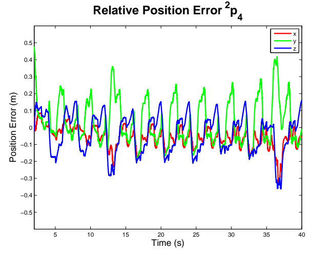
Fig. 8. The relative position error {}^2p_4 .
