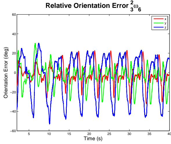
Fig. 5. The relative orientation error {}^2_3\omega_6 .
