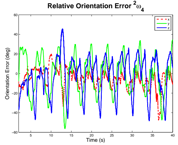
Fig. 9. The relative position error {}^2\omega_4 .
