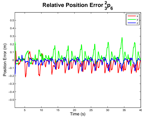
Fig. 4. The relative position error {}^2_3p_6 .
