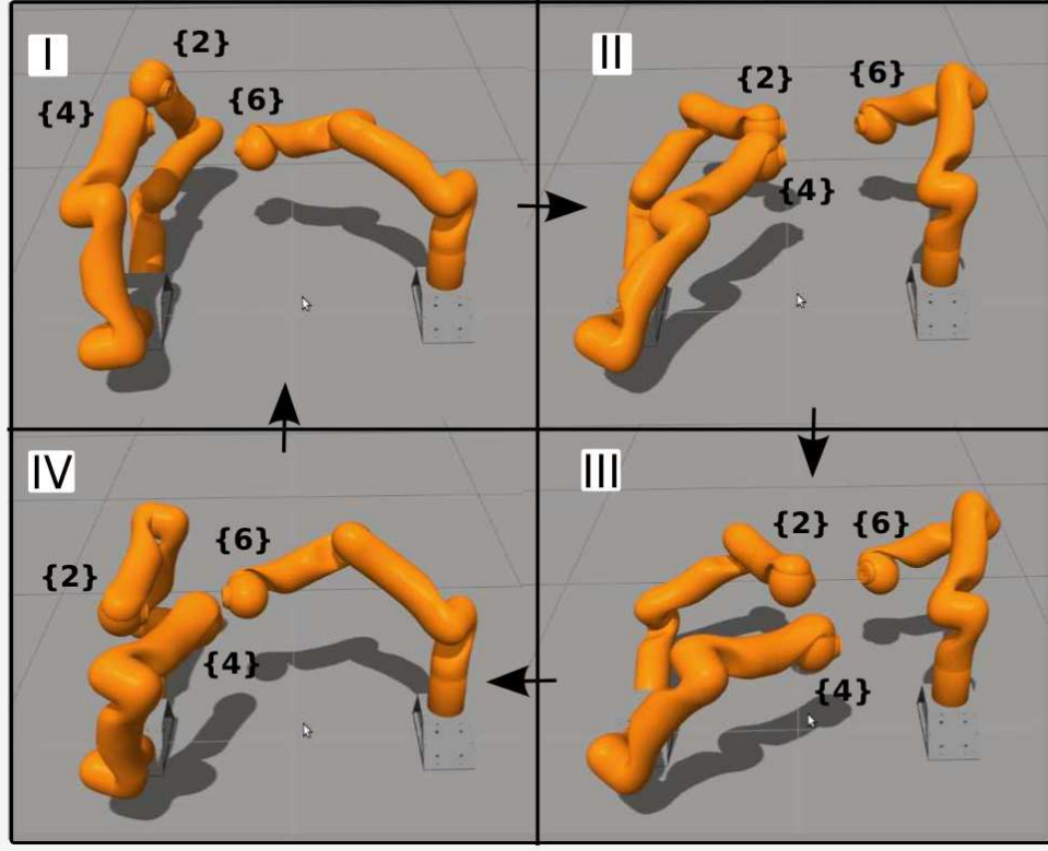
Fig. 3. Snapshots of Gazebo simulation where the 3-arm parallel manipulators move in a coordinated manner, in single manipulator control.
